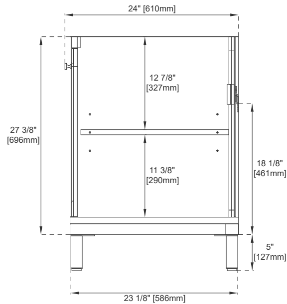
Side View 2
