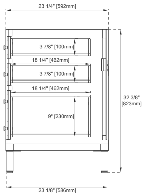
Side View 1
