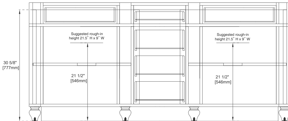
Back View
