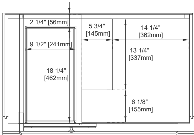
Top View 1
