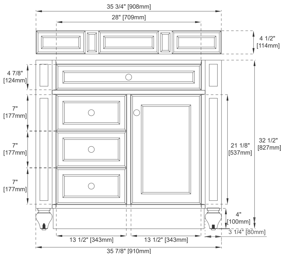
Front View
