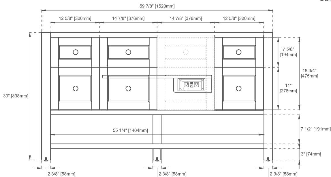
Front View
