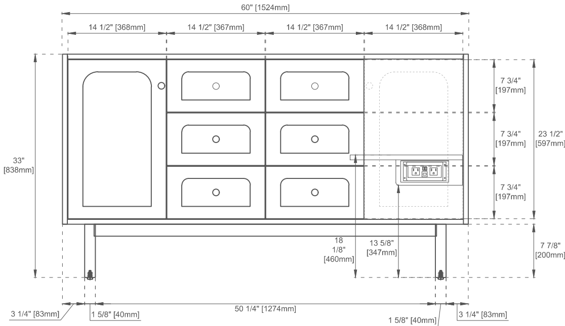
Front View
