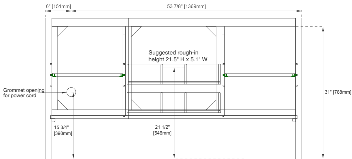
Back View
