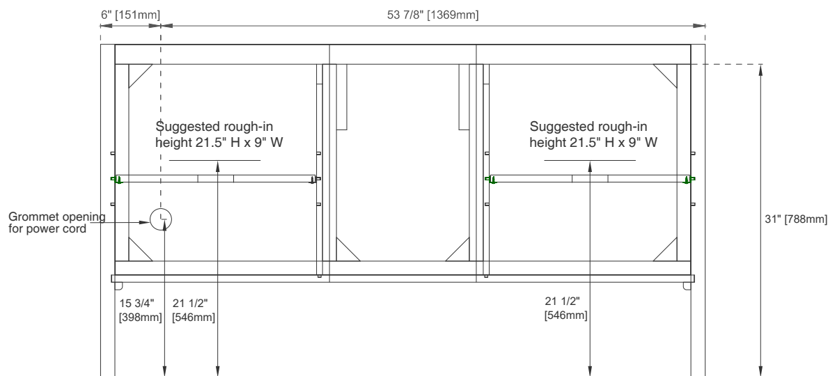
Back View
