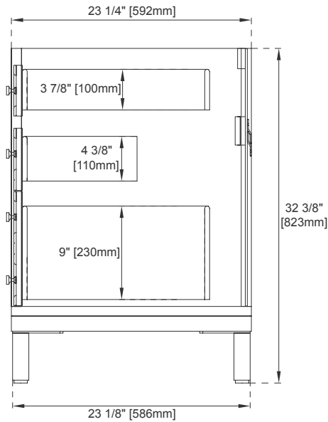
Side View 1
