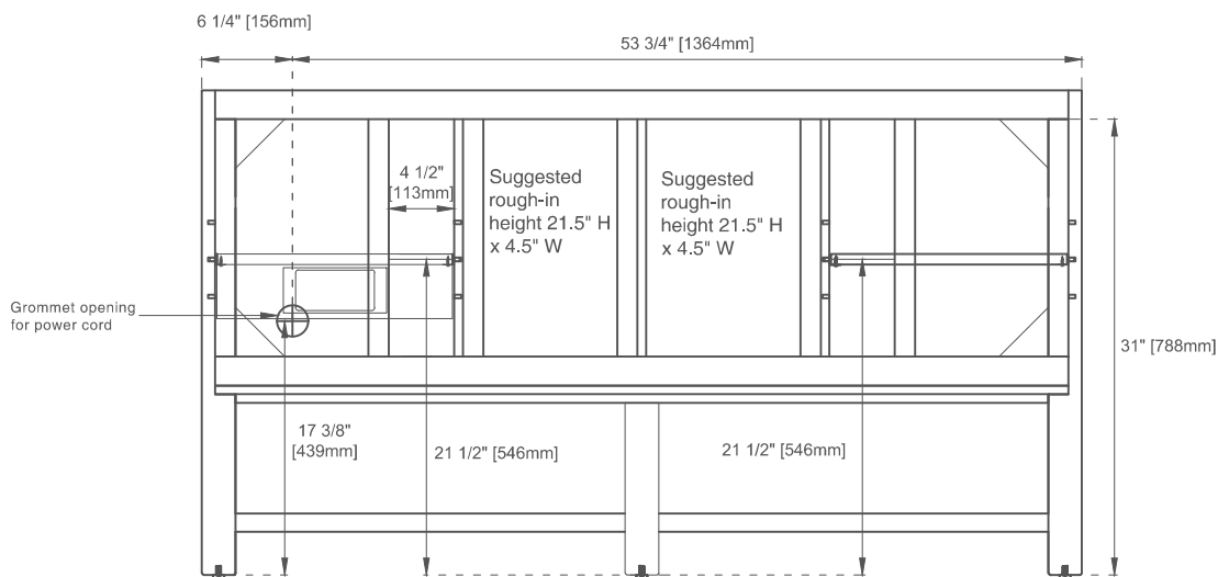
Back View
