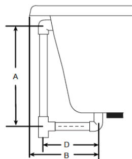
Drain/Overflow
