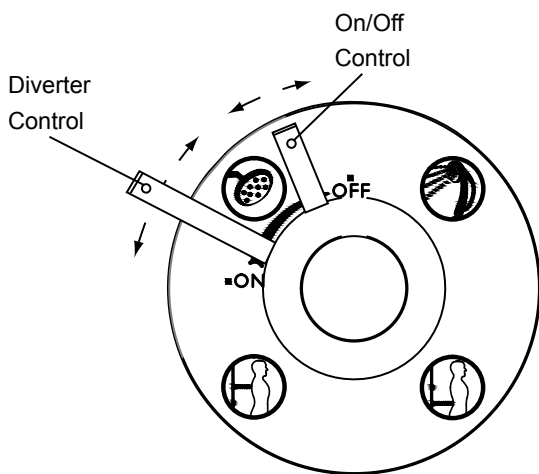
4-Port Diverter Valve (For Package A Units Only)
