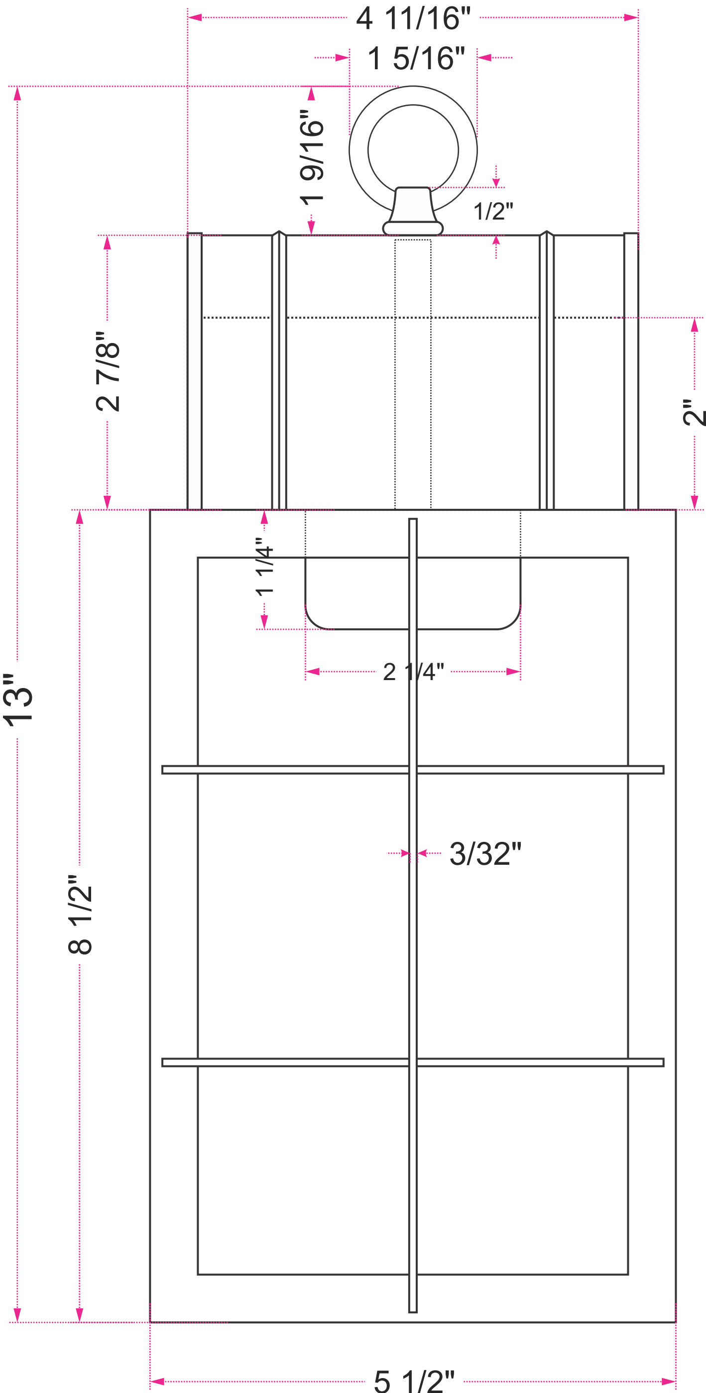
Front View
