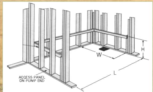
Framing Dimensions
