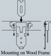
Mounting on Wood Frame
