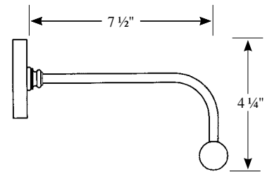
DSL36" shade six 15T4 bulbs included
