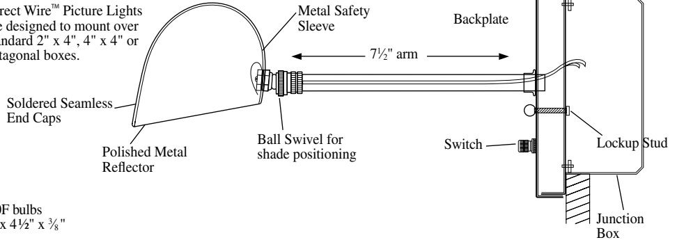
DT24" shade three 25 or 40T10F bulbs Backplate: 4" x 15" x ⅜"
