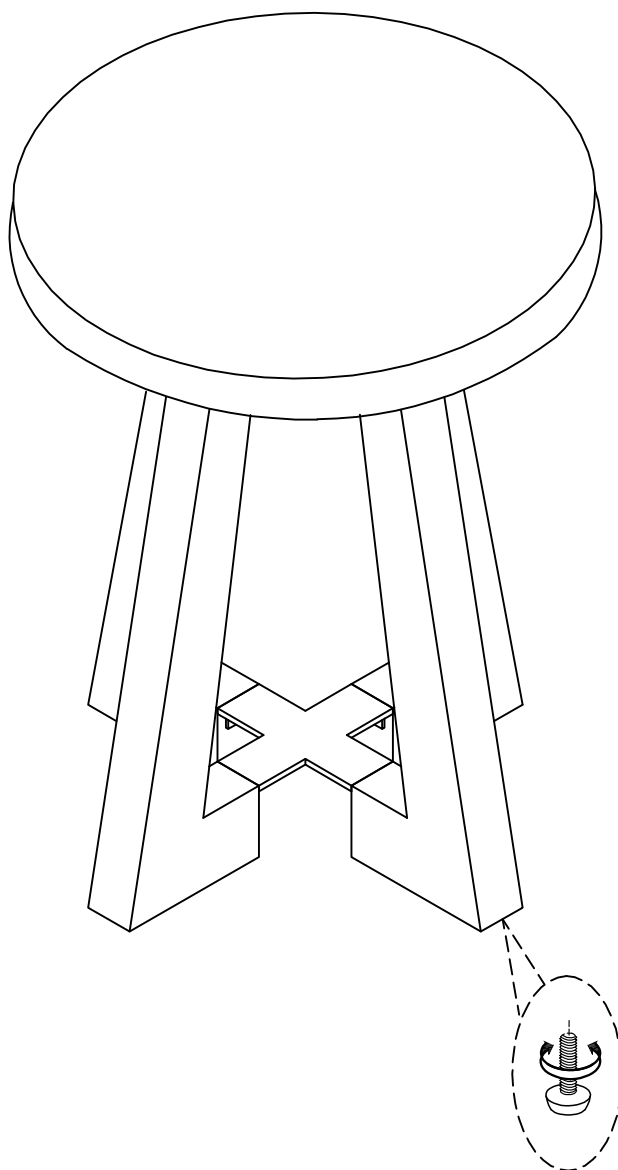
Adjustable leveler
