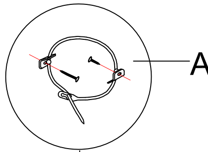
Tipping Restraint
