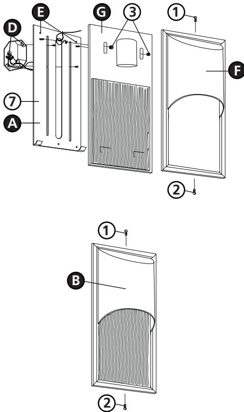
Drawing 1 - Fixture Mounting
