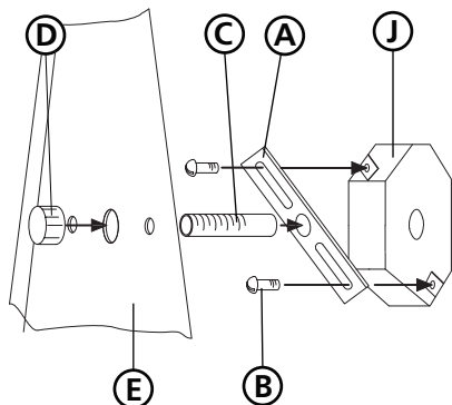
Drawing 1 - Fixture Mounting
