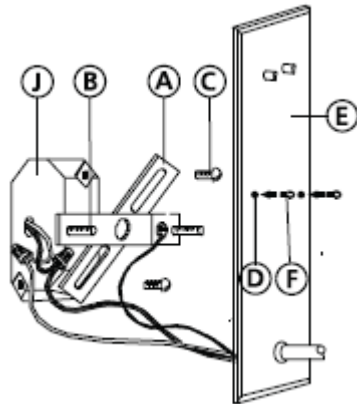
Drawing 2 – Glass Replacement
