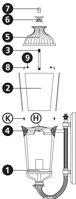
Drawing 3 - Glass Installation
