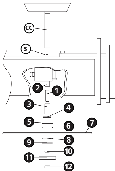
Drawing 2 - Strap Detail
