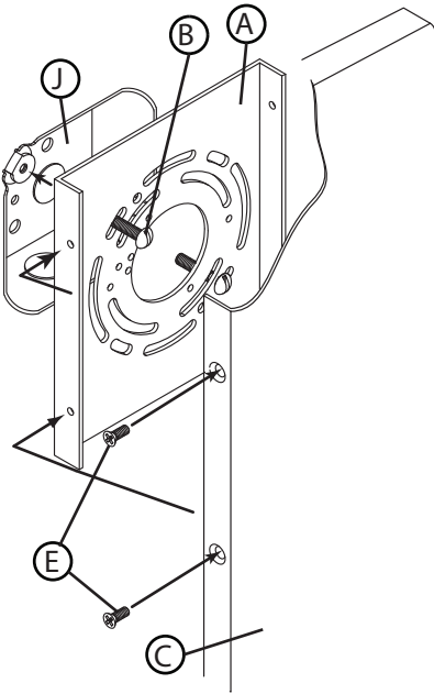
Drawing 1- Fixture Mounting
