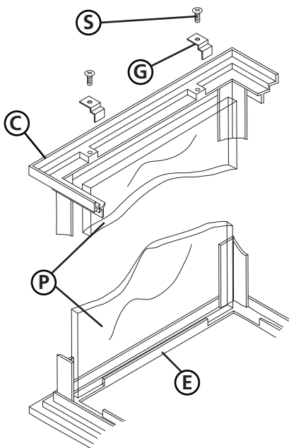
DRAWING 2 - MOUNTING
