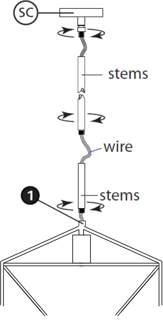
Drawing 2 – Strap Detail
