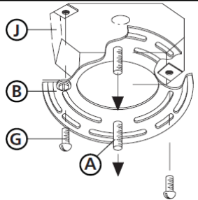
Drawing 3 – Fixture Mounting
