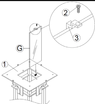
Drawing 3 – Fixture Mounting
