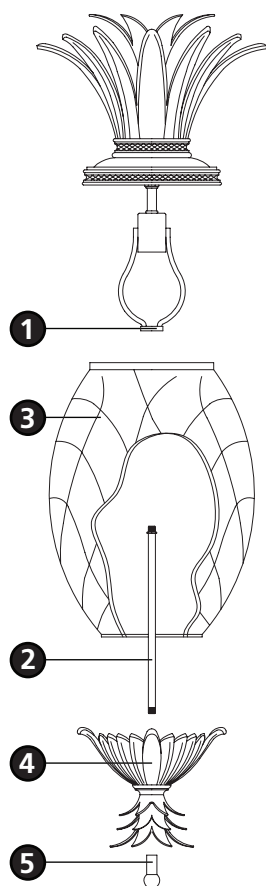
Drawing 1 - Fixture Assembly
