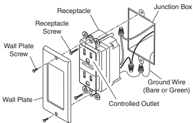
Installing Receptacle Receiver
