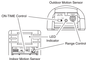
Indoor Motion Sensor
