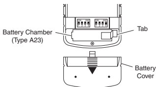
Rear View of Remote Control
