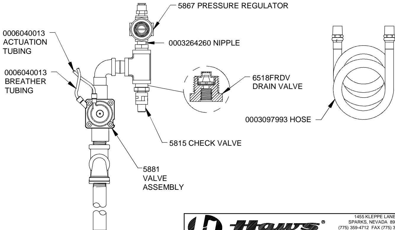
VRK3AV DETAIL 1
