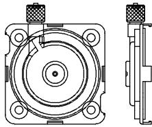
VRK3AV DETAIL 1
