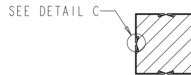
SECTION A-A SCALE 1:8
