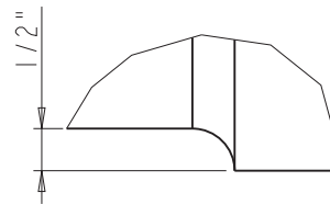
DETAIL A SCALE 2:5
