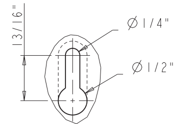
DETAIL A SCALE 3:5
