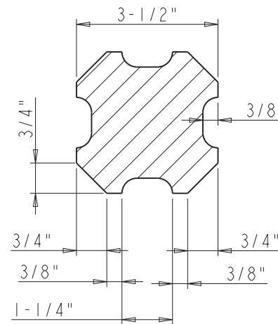
SECTION A-A SCALE 3:10
