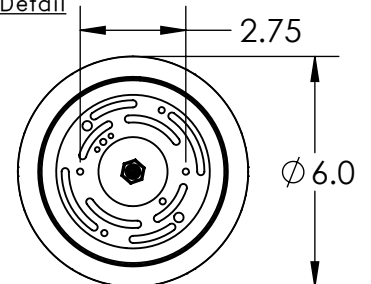
Mounting Detail
