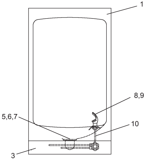
FIG. 5 FRONT PANEL
