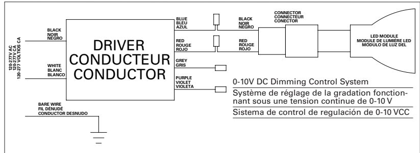
Figure 5. Electrical Connection
