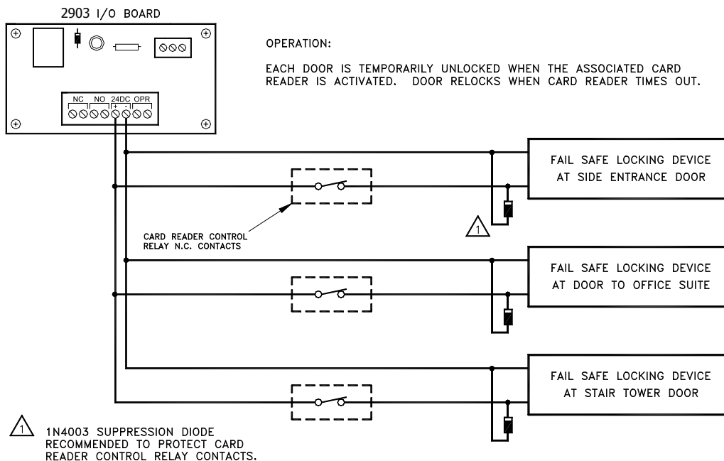
Figure 4 Wire scheme for independent control of multiple doors
