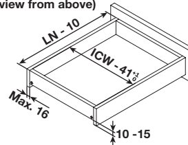
Drawer with front (view from above)
