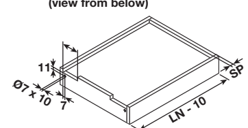
Drawer drilling (view from below)
