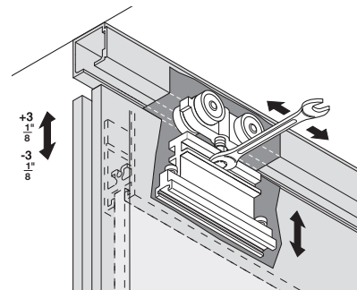
Height adjustment
