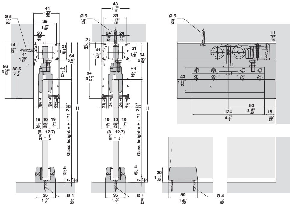
Ceiling Mounted
