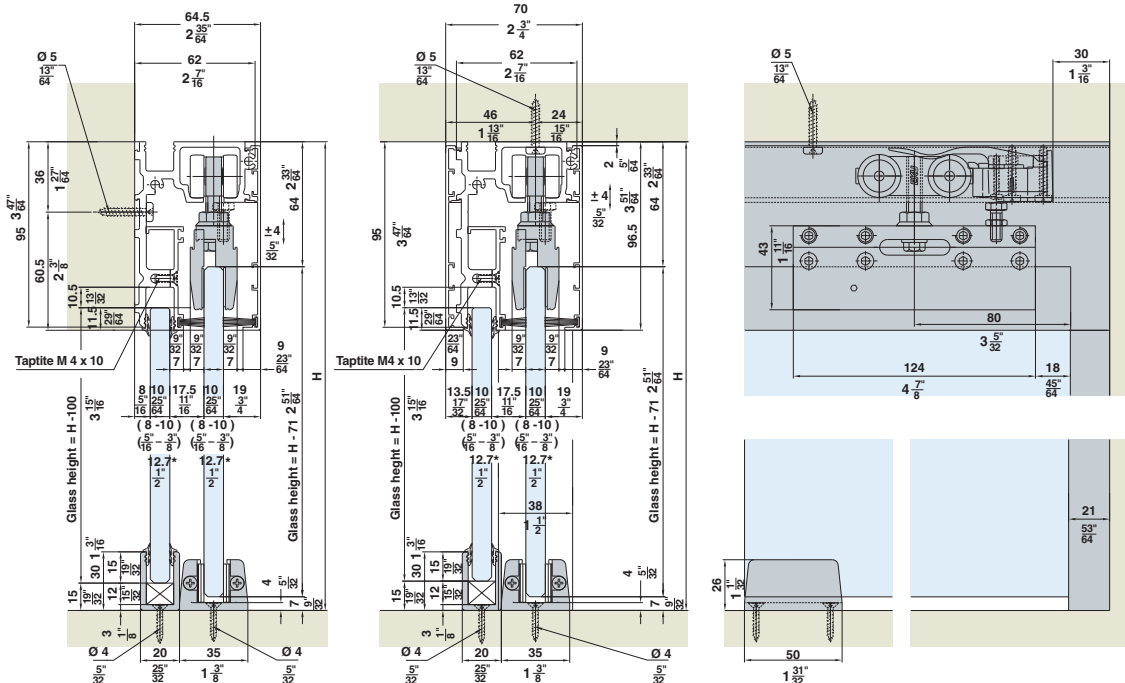
Wall Mounted
