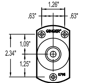
MOUNTING FLANGE DETAIL
