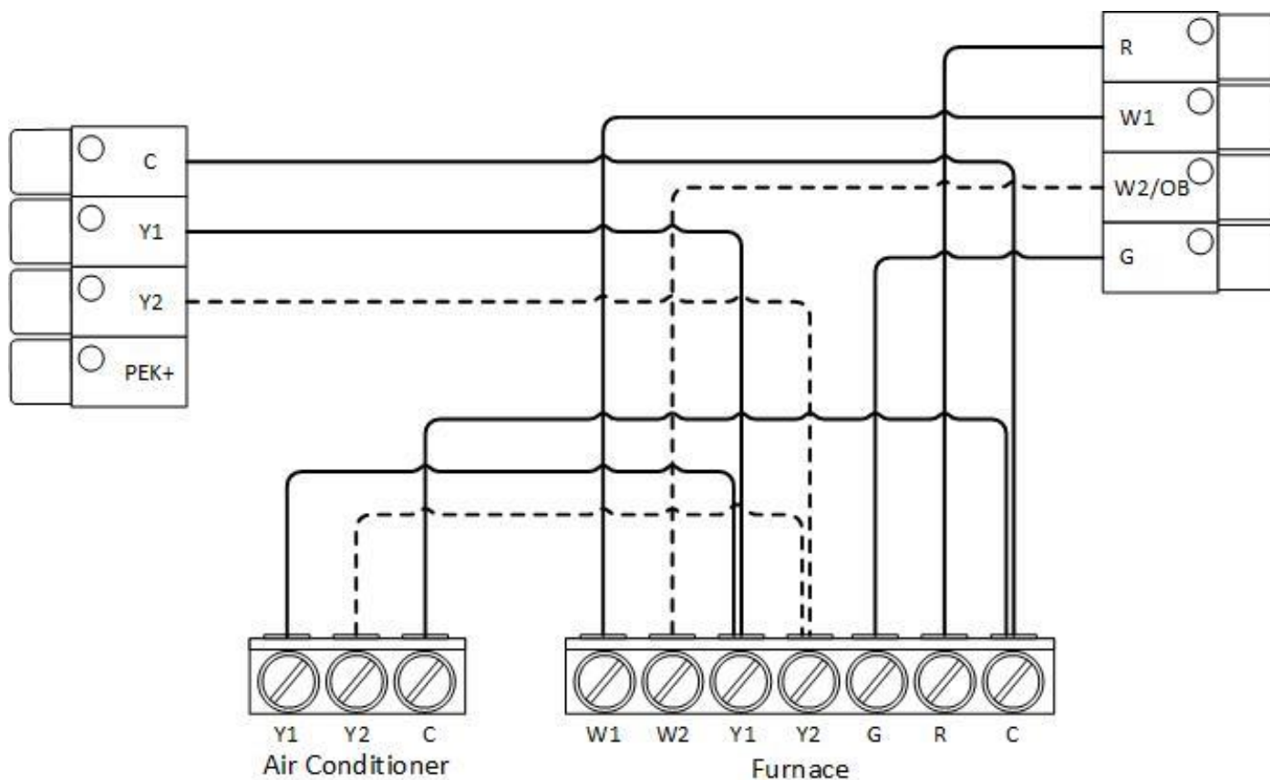
Diagram 1. Conventional HVAC systems (up to 2-heat/2-cool)
