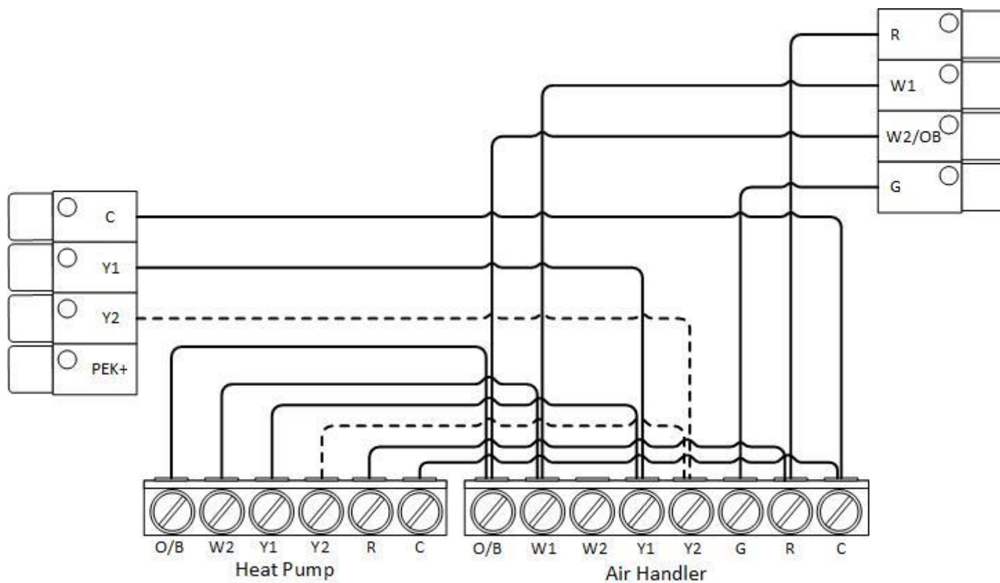
Diagram 3. Heatpump systems (up to 3-heat/2-cool)
