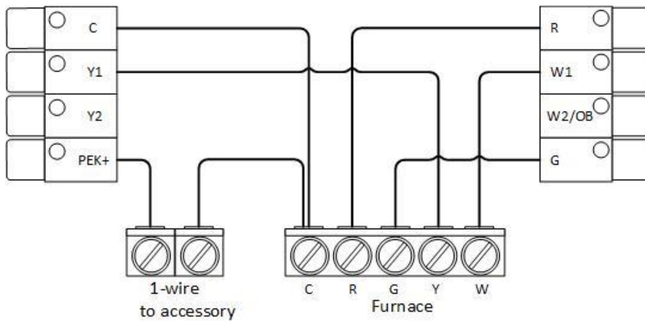
Diagram 10. 1-wire HVAC accessory using PEK+
