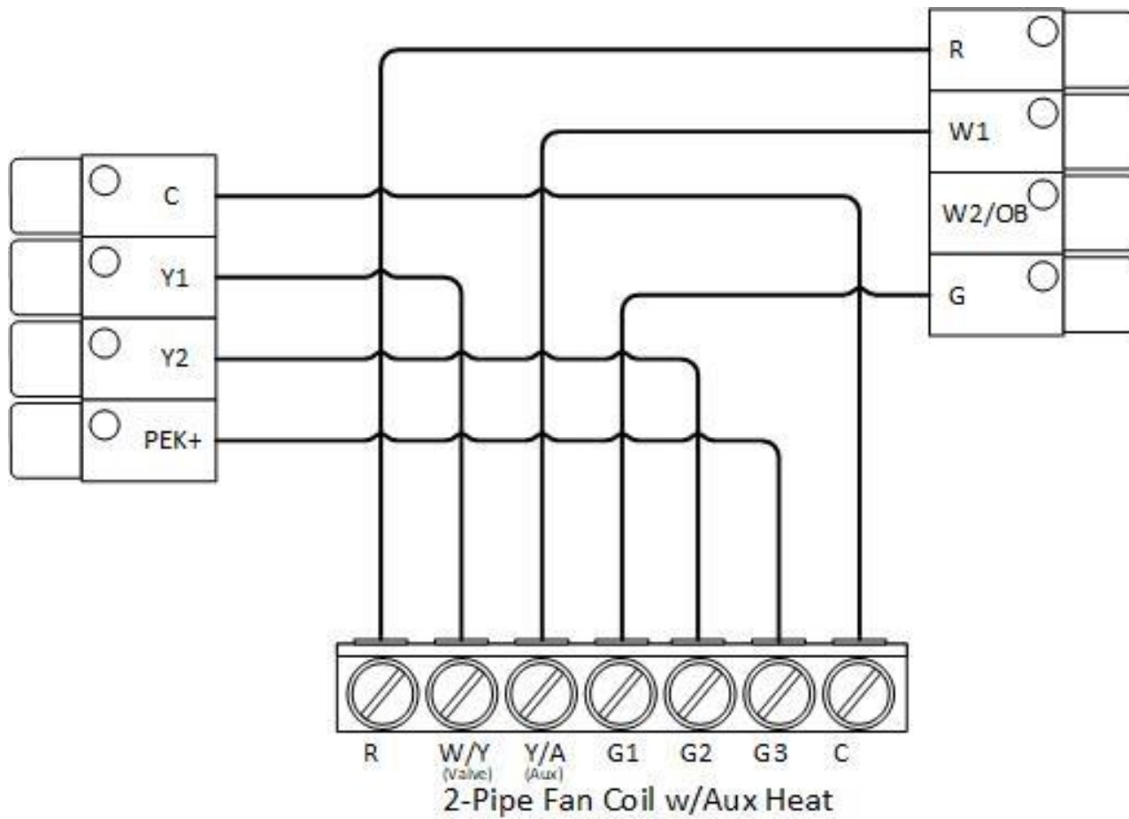
Diagram 6. Multi-speed fan 2-pipe fan coil with Aux Heat.
