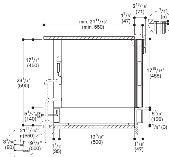
Side view of WS 461 below BS Combi-steam oven, BM Combi-microwave oven or CM espresso machine
