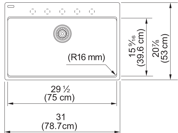
Dimensional Drawing
