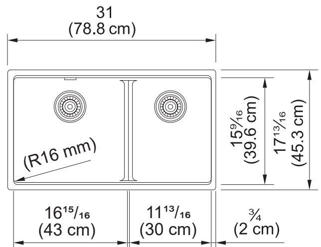
Dimensional Drawing
