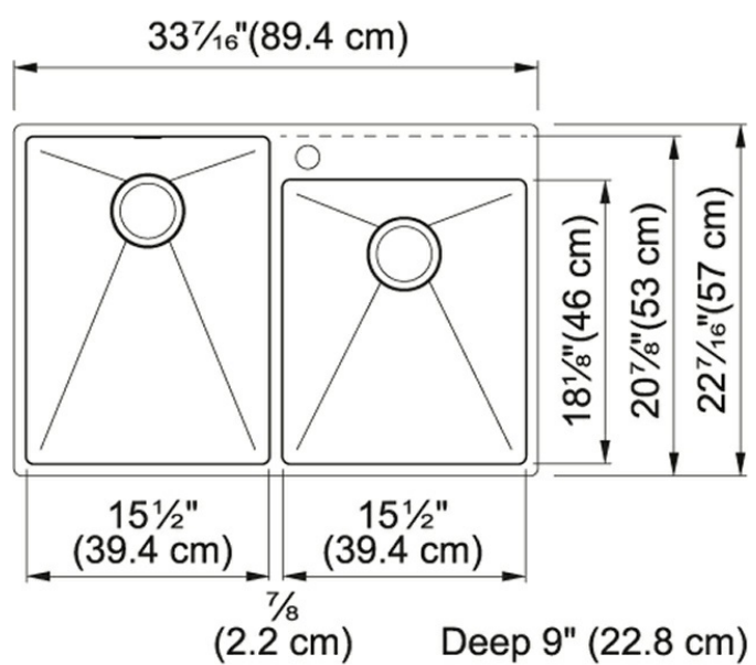
Technical Drawing
