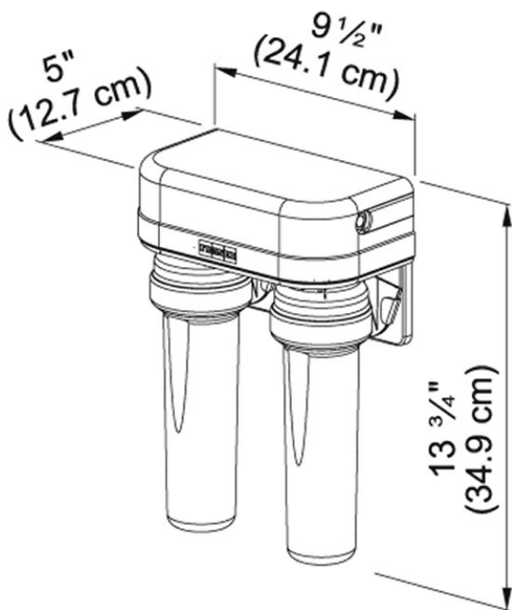
Technical Drawing
