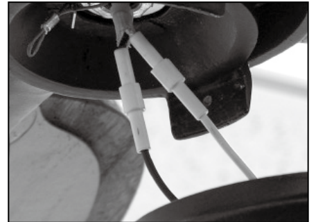
3. Connect white-to-white and blue-to-black wires.
