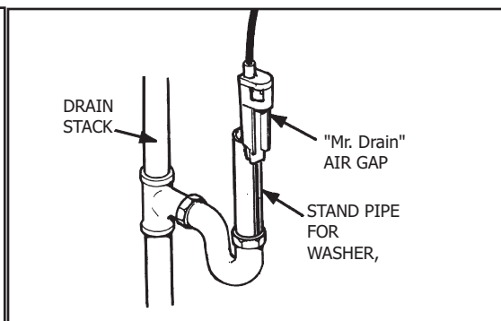
Air Gap - "Mr. Drain"
