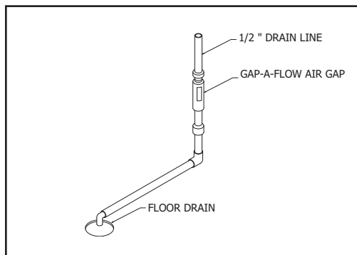
Air Gap - Floor Drain
