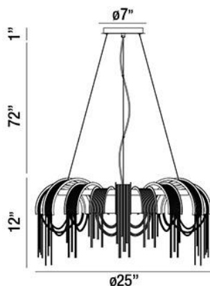
Draped nickel chain wrapped around curved nickel strips
